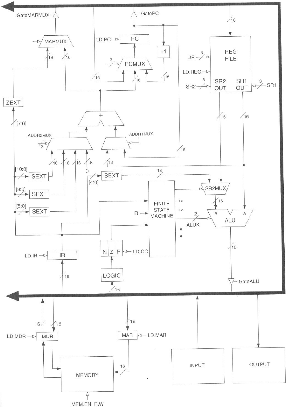
Figure 3.33 The data path of the LC-3 computer
